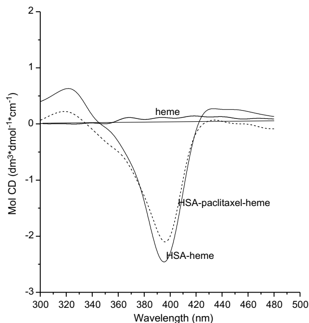
Figure 4. Effect of paclitaxel on the visible CD spectrum of HSA–heme complex. Molar ratio of heme/protein, 2:1. Concentration of HSA, 8 \times 10^{-6} M, paclitaxel–HSA was incubated 24 h at 37 °C at molar ratio 10:1. Mol CD units are \text{dm}^3 \text{mol}^{-1} \text{cm}^{-1} .
