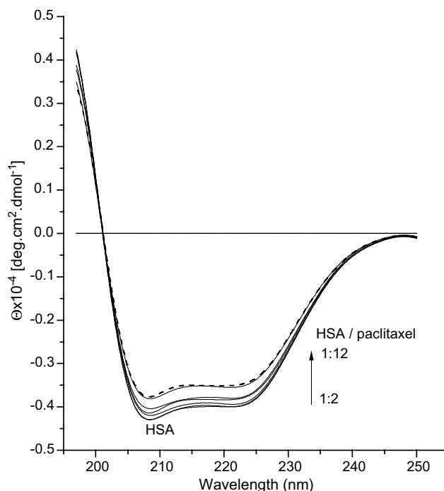
Figure 1. The effect of paclitaxel concentration on CD spectra of HSA. Concentration of HSA, 8 \times 10^{-6} \text{ M} , paclitaxel–HSA was incubated 24 h at 37 °C at molar ratio from 2:1 to 12:1.
