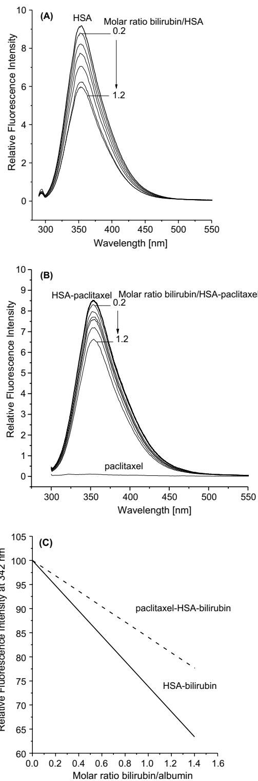
Figure 7. Fluorescence quench titration results of HSA (A) and HSA-paclitaxel (B) at increasing bilirubin to protein molar ratios obtained in phosphate buffer pH 7.4. The molar ratio was varied from 0.2 to 1.2 in each case and the excitation and emission wavelengths were 295 and 342 nm, respectively. The data were plotted as percent fluorescence versus bilirubin to protein molar ratio (C). Concentration of HSA: 8 \times 10^{-6} M, paclitaxel was incubated with HSA 24 h at 37 °C at molar ratio paclitaxel/HSA, 10:1.
