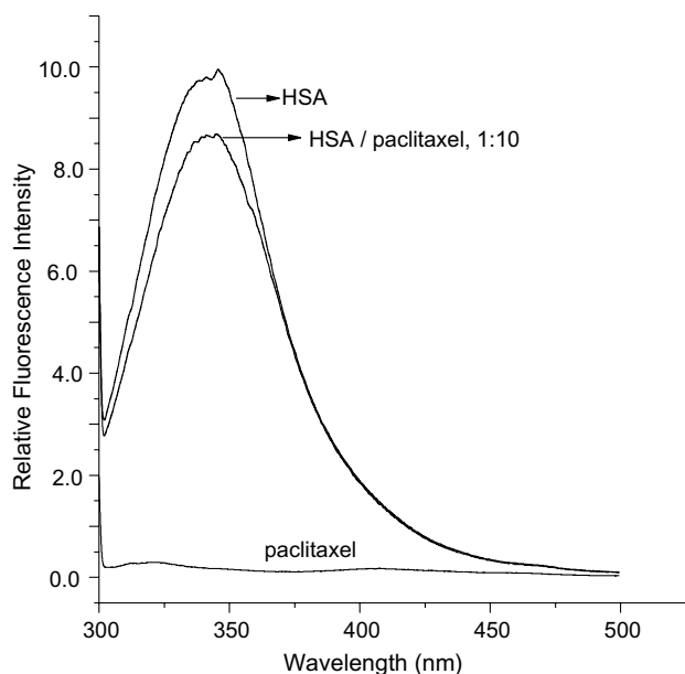
Figure 2. Tryptophan fluorescence spectral changes of HSA incubated with paclitaxel. The molar ratio paclitaxel/HSA, 10:1. The excitation and emission wavelengths were 295 and 342 nm, respectively. Concentration of HSA, 8 \times 10^{-6} M, paclitaxel–HSA was incubated 24 h at 37 °C.
