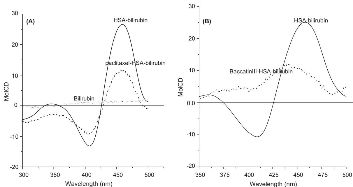
Figure 5. Effect of paclitaxel (A) and baccatin III (B) on the visible CD spectrum of HSA–bilirubin complex. Molar ratio of bilirubin/protein, 2:1. Concentration of HSA, 8 \times 10^{-6} M, paclitaxel–HSA and baccatin III–HSA were incubated 24 h at 37 °C at molar ratio 10:1. Mol CD units are \text{dm}^3 \text{mol}^{-1} \text{cm}^{-1} .
