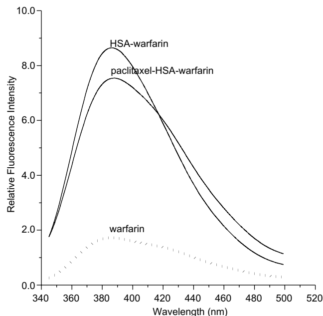
Figure 3. Relative fluorescence changes of warfarin with paclitaxel-treated HSA. Excitation at 335 nm and emission at 378 nm. Warfarin was incubated for 1 h at 37 °C with HSA and paclitaxel–HSA at molar ratio warfarin/protein 1:1. Concentration of HSA: 4 \times 10^{-6} M, paclitaxel–HSA was incubated 24 h at 37 °C at molar ratio 10:1.
